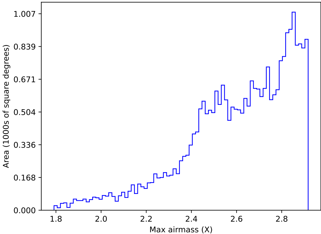
ddf_loaded_half_fl1_v3.4_10yrs All sky all bands: Max airmass
