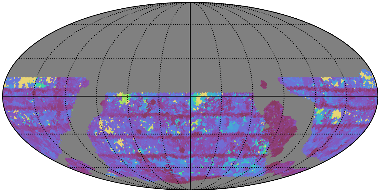
ddf_loaded_half_fl1_v3.4_10yrs WFD z band: Max Inter-Night Gap
