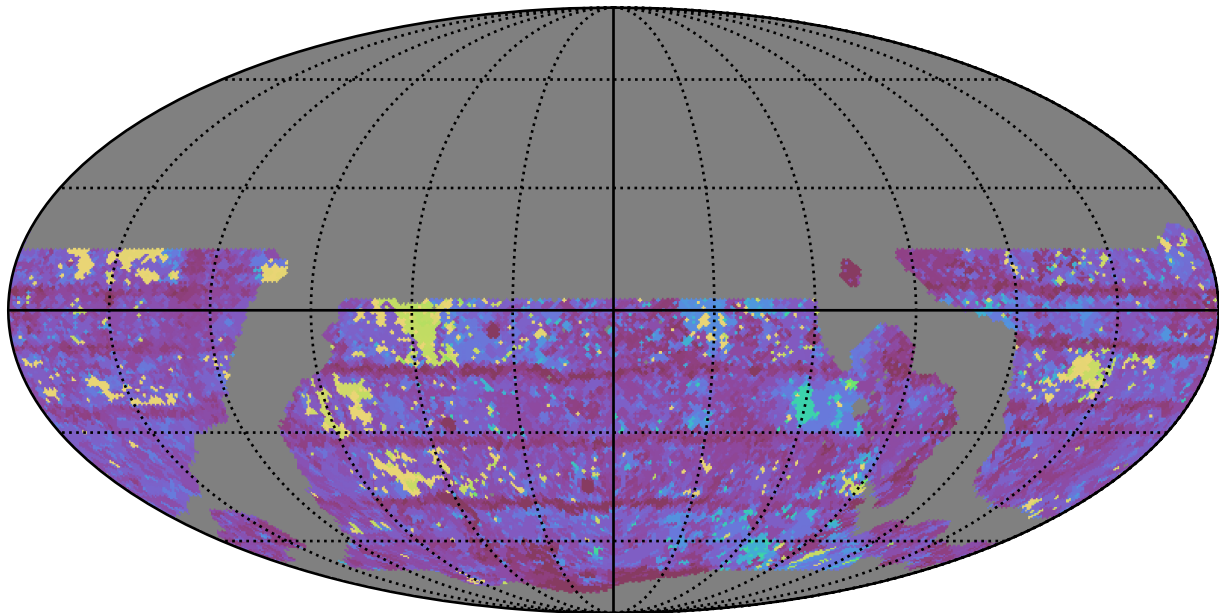
ddf_loaded_half_fl1_v3.4_10yrs WFD y band: Max Inter-Night Gap
