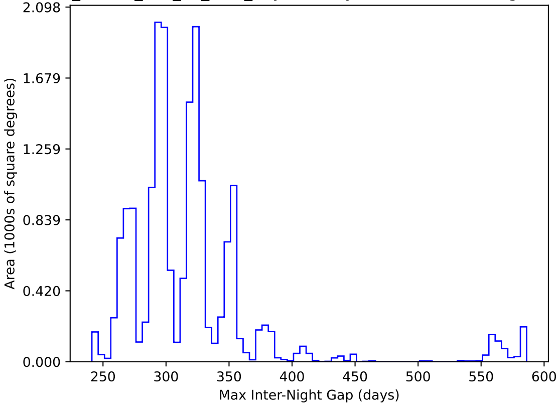
ddf_loaded_half_fl1_v3.4_10yrs WFD y band: Max Inter-Night Gap
