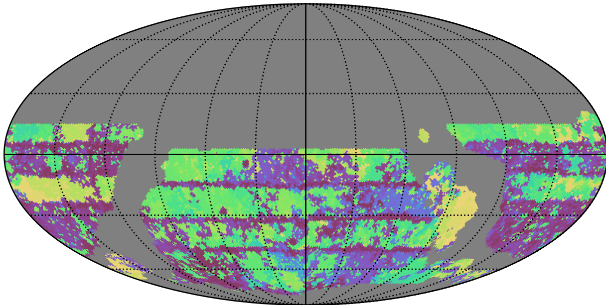
ddf_loaded_half_fl1_v3.4_10yrs WFD u band: Max Inter-Night Gap
