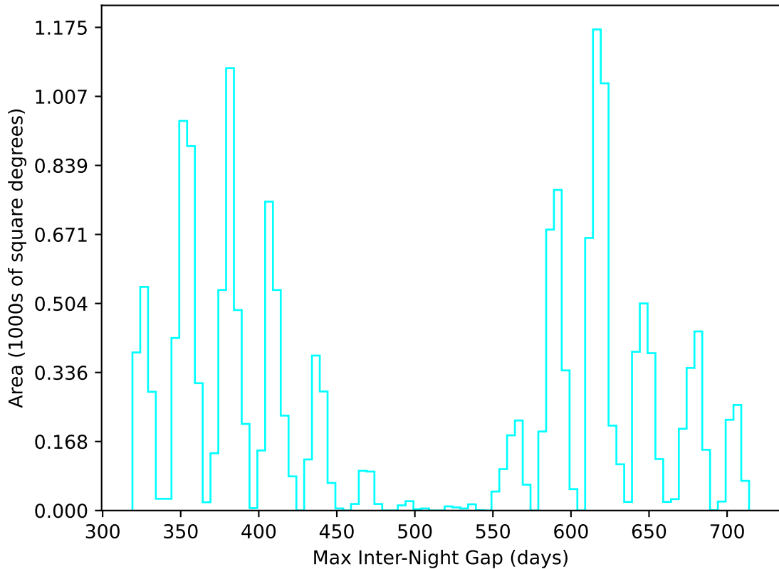
ddf_loaded_half_fl1_v3.4_10yrs WFD u band: Max Inter-Night Gap
