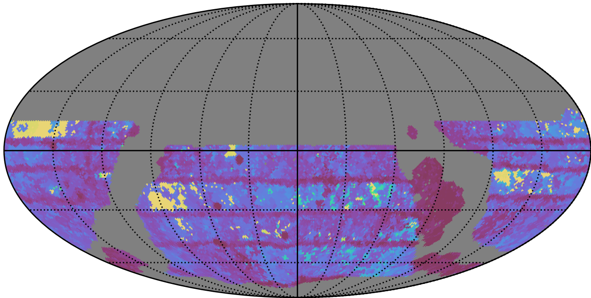
ddf_loaded_half_fl1_v3.4_10yrs WFD r band: Max Inter-Night Gap
