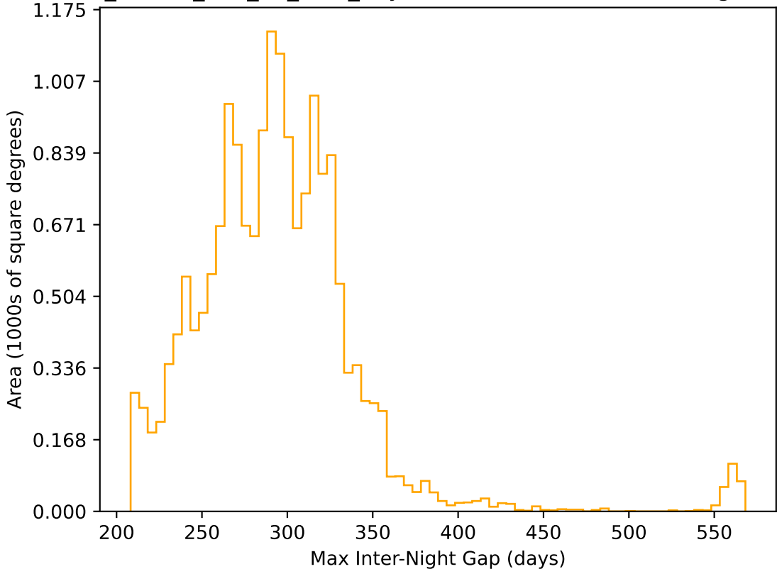
ddf_loaded_half_fl1_v3.4_10yrs WFD r band: Max Inter-Night Gap
