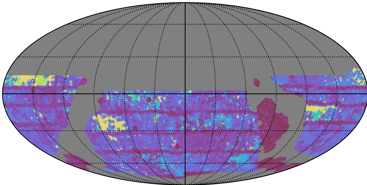
ddf_loaded_half_fl1_v3.4_10yrs WFD i band: Max Inter-Night Gap
