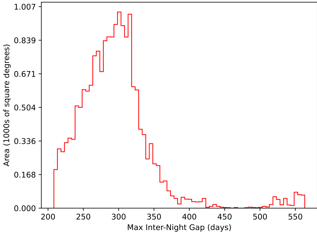
ddf_loaded_half_fl1_v3.4_10yrs WFD i band: Max Inter-Night Gap
