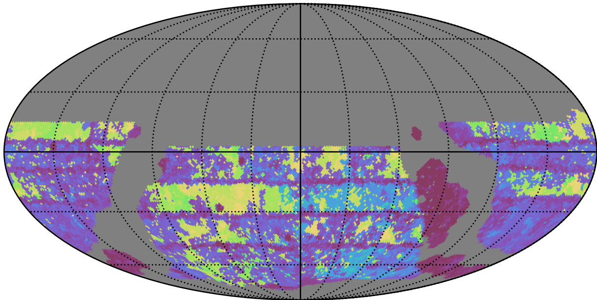
ddf_loaded_half_fl1_v3.4_10yrs WFD g band: Max Inter-Night Gap
