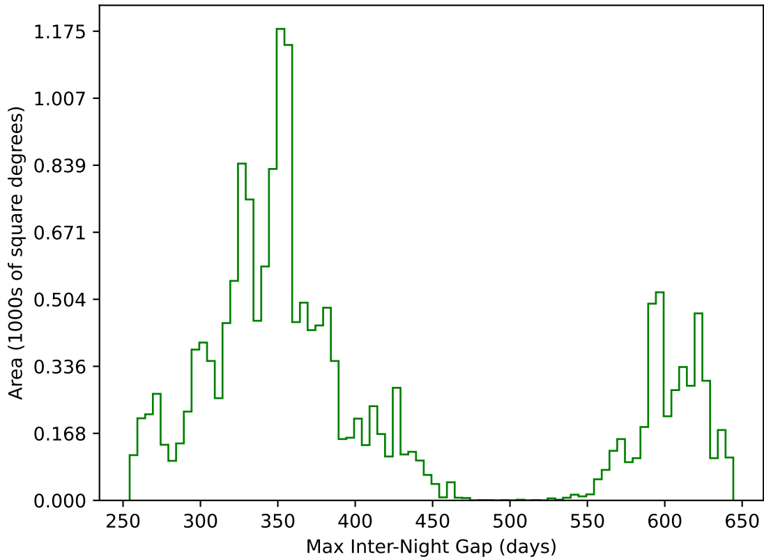
ddf_loaded_half_fl1_v3.4_10yrs WFD g band: Max Inter-Night Gap
