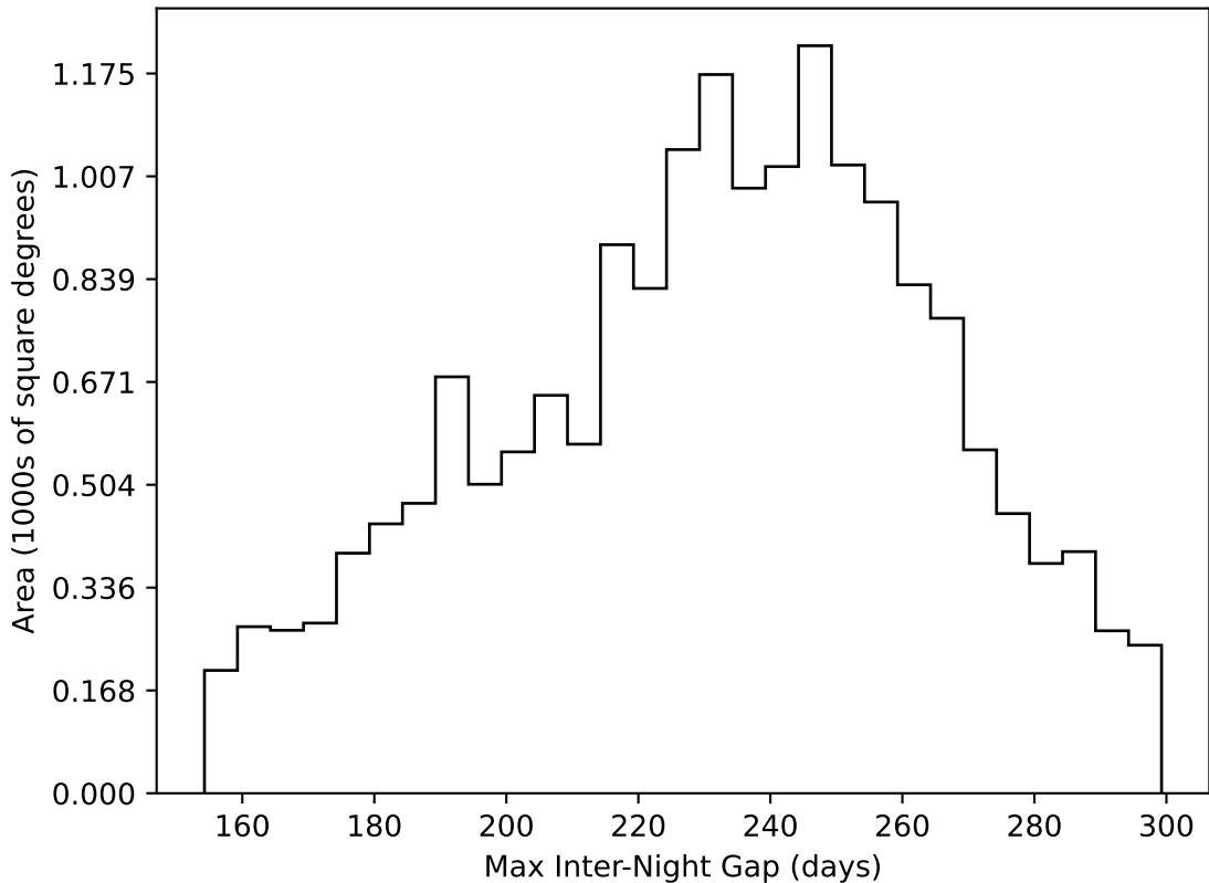
ddf_loaded_half_fl1_v3.4_10yrs WFD all bands: Max Inter-Night Gap
