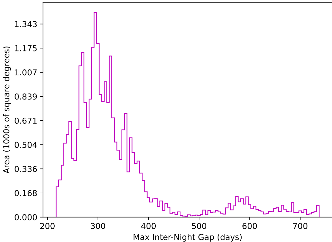
ddf_loaded_half_fl1_v3.4_10yrs All sky z band: Max Inter-Night Gap
