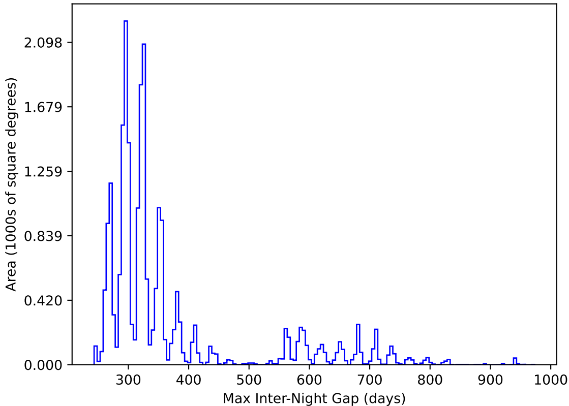
ddf_loaded_half_fl1_v3.4_10yrs All sky y band: Max Inter-Night Gap
