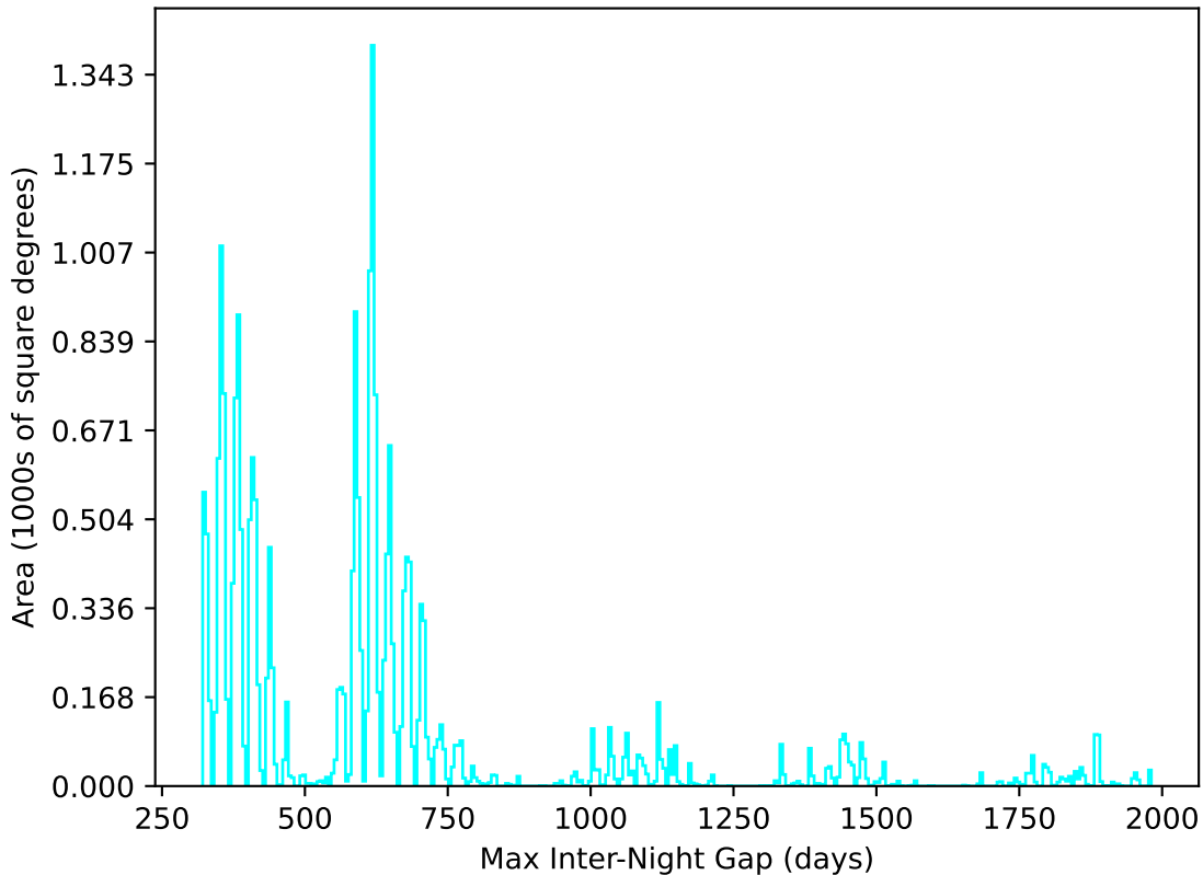
ddf_loaded_half_fl1_v3.4_10yrs All sky u band: Max Inter-Night Gap
