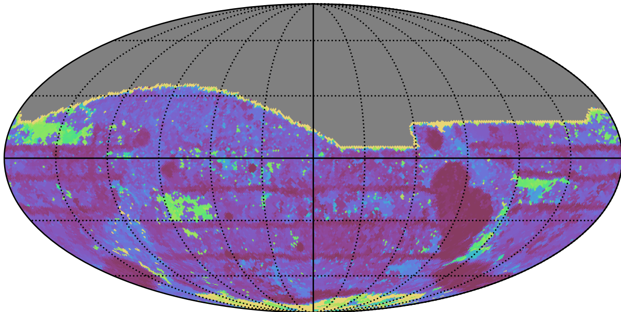
ddf_loaded_half_fl1_v3.4_10yrs All sky i band: Max Inter-Night Gap
