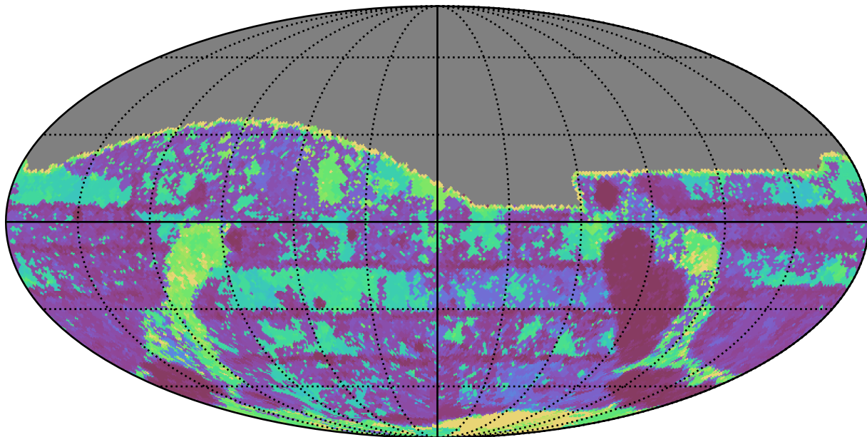
ddf_loaded_half_fl1_v3.4_10yrs All sky g band: Max Inter-Night Gap
