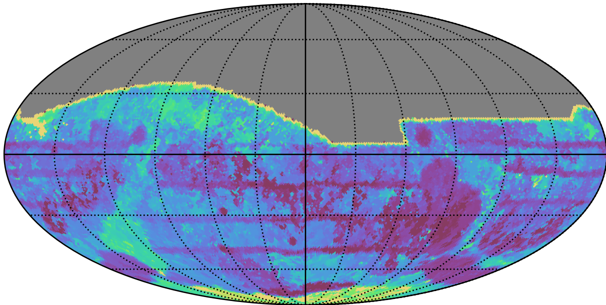
ddf_loaded_half_fl1_v3.4_10yrs All sky all bands: Max Inter-Night Gap
