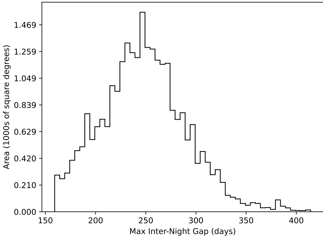
ddf_loaded_half_fl1_v3.4_10yrs All sky all bands: Max Inter-Night Gap
