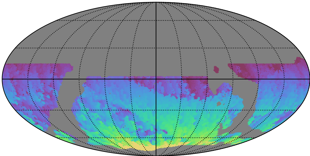
ddf_loaded_half_fl1_v3.4_10yrs WFD z band: Max HA
