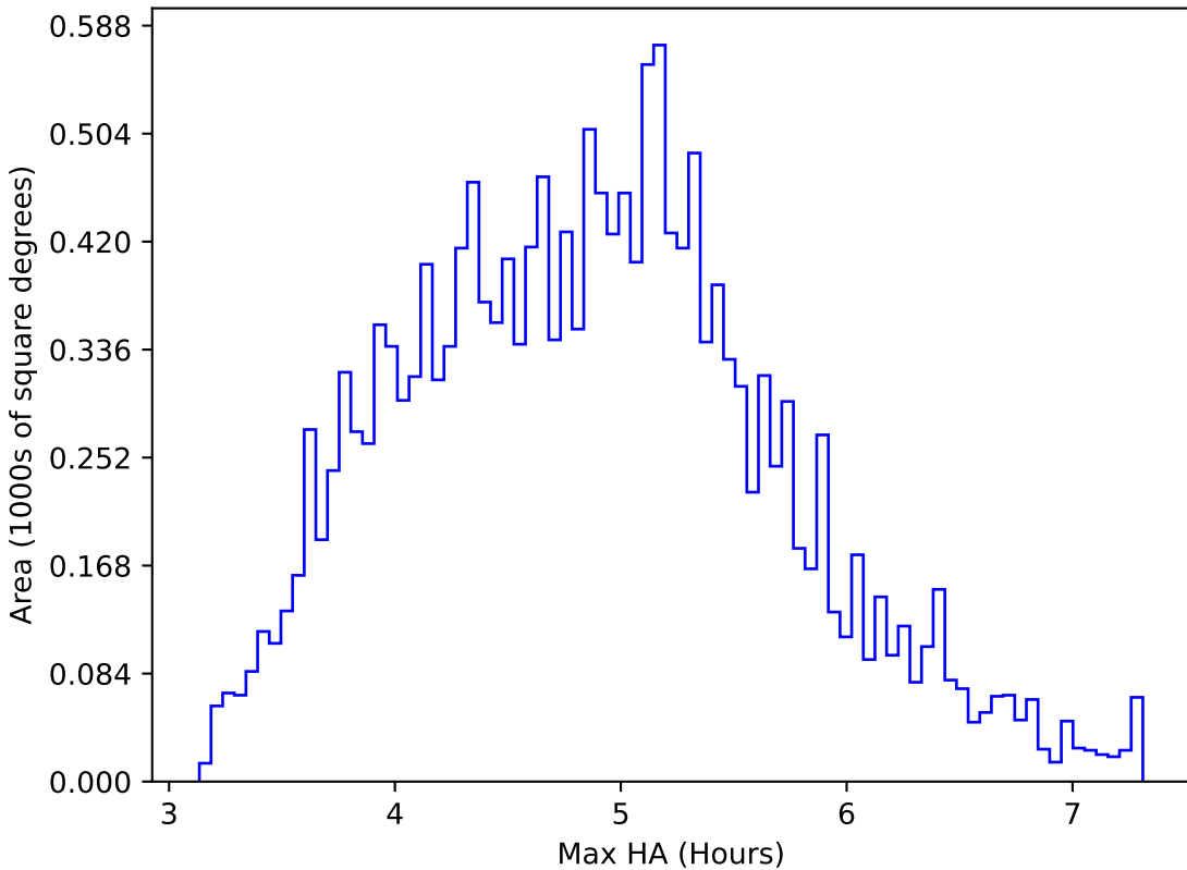
ddf_loaded_half_fl1_v3.4_10yrs WFD z band: Max HA
