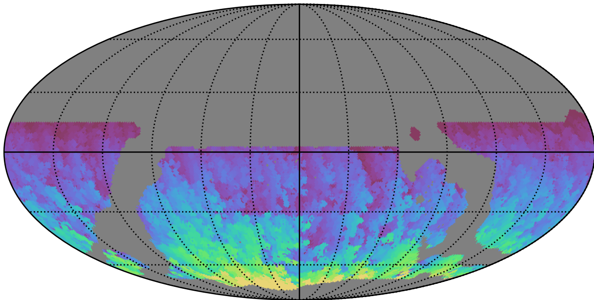
ddf_loaded_half_fl1_v3.4_10yrs WFD y band: Max HA
