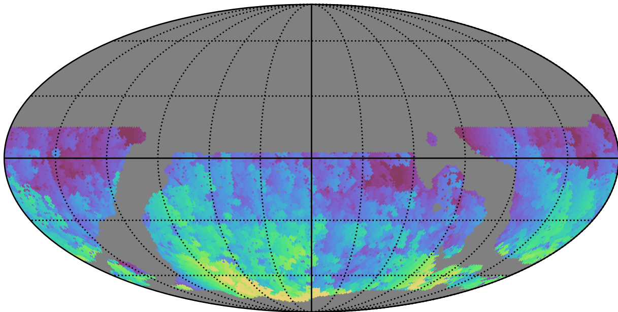
ddf_loaded_half_fl1_v3.4_10yrs WFD u band: Max HA
