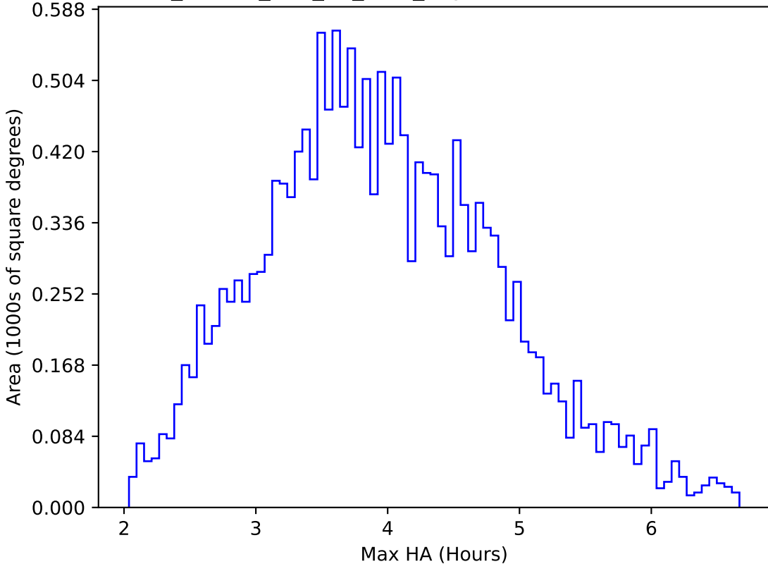
ddf_loaded_half_fl1_v3.4_10yrs WFD u band: Max HA
