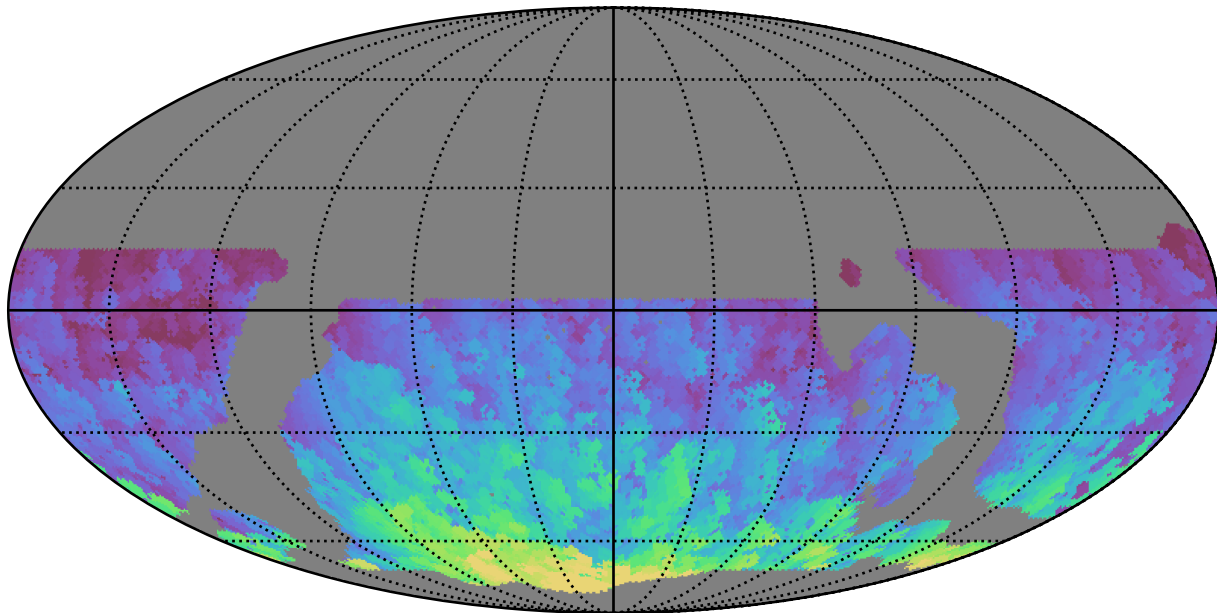
ddf_loaded_half_fl1_v3.4_10yrs WFD r band: Max HA
