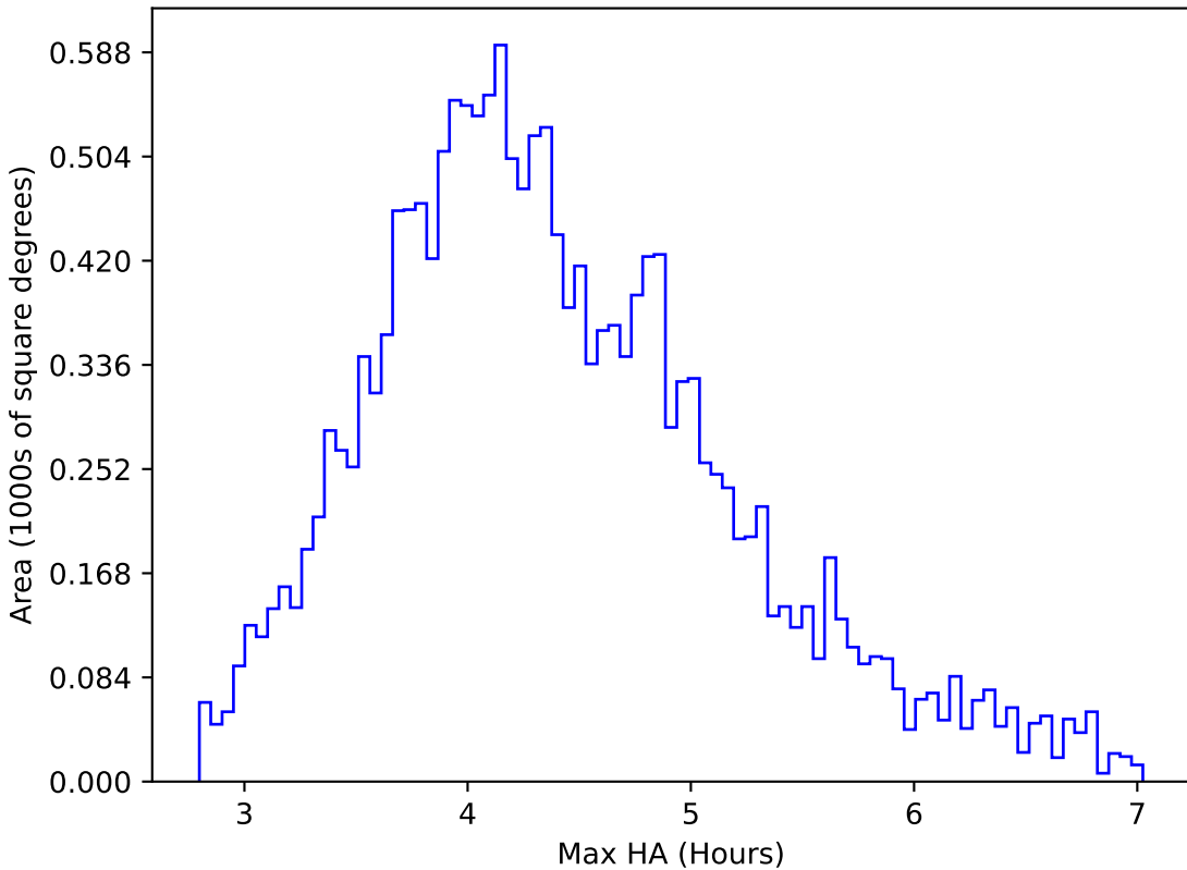
ddf_loaded_half_fl1_v3.4_10yrs WFD r band: Max HA
