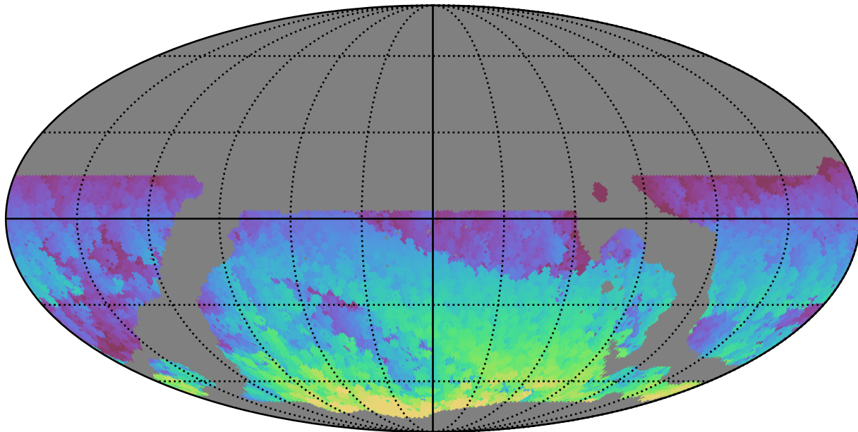
ddf_loaded_half_fl1_v3.4_10yrs WFD i band: Max HA
