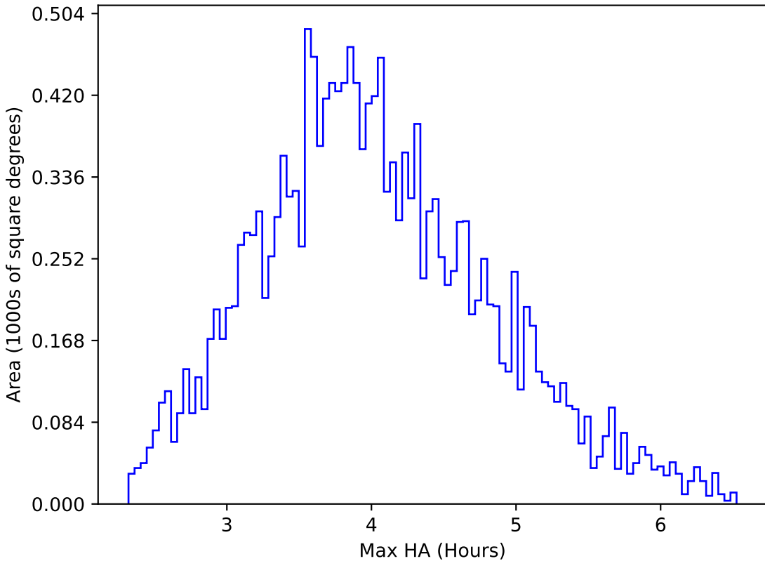
ddf_loaded_half_fl1_v3.4_10yrs WFD g band: Max HA
