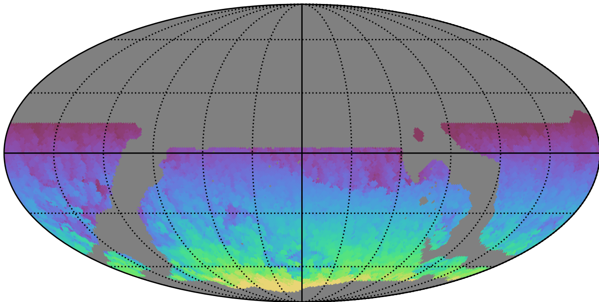
ddf_loaded_half_fl1_v3.4_10yrs WFD all bands: Max HA
