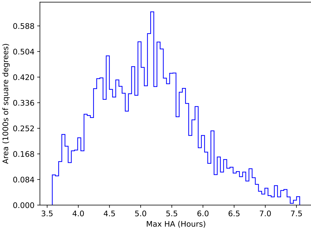
ddf_loaded_half_fl1_v3.4_10yrs WFD all bands: Max HA
