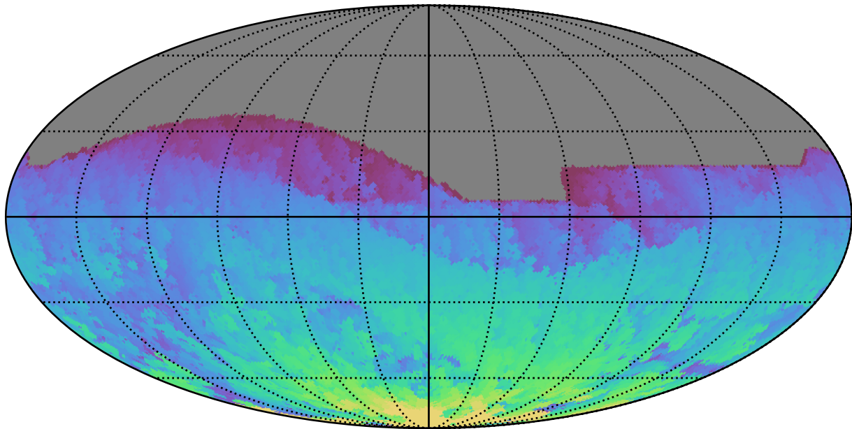
ddf_loaded_half_fl1_v3.4_10yrs All sky z band: Max HA
