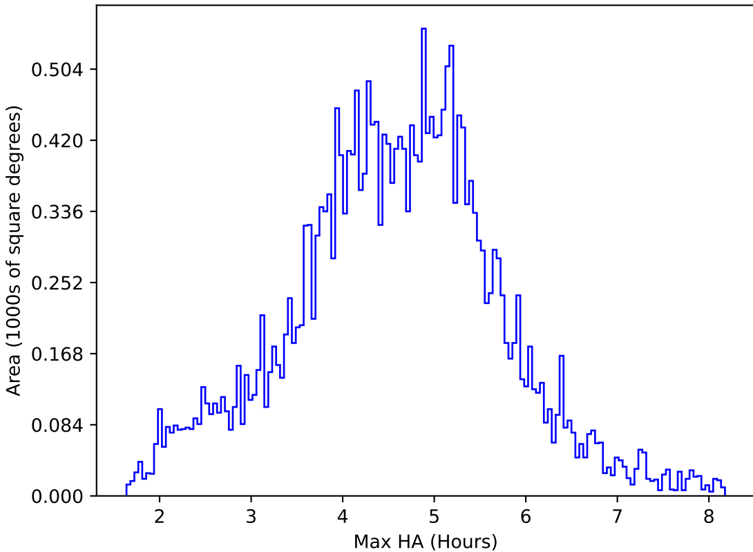
ddf_loaded_half_fl1_v3.4_10yrs All sky z band: Max HA
