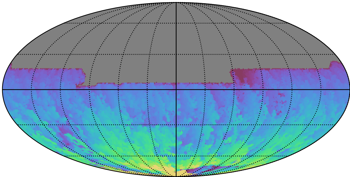
ddf_loaded_half_fl1_v3.4_10yrs All sky y band: Max HA
