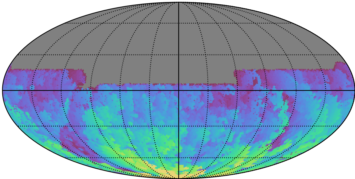
ddf_loaded_half_fl1_v3.4_10yrs All sky u band: Max HA
