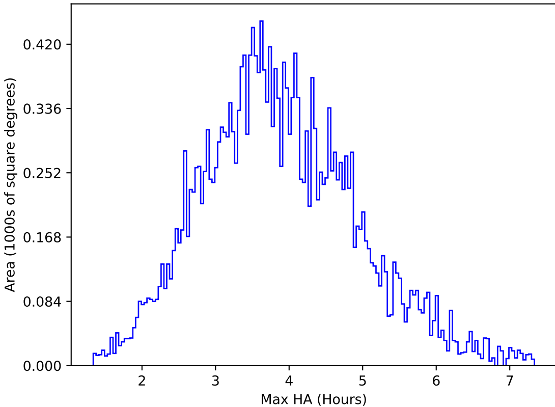
ddf_loaded_half_fl1_v3.4_10yrs All sky u band: Max HA
