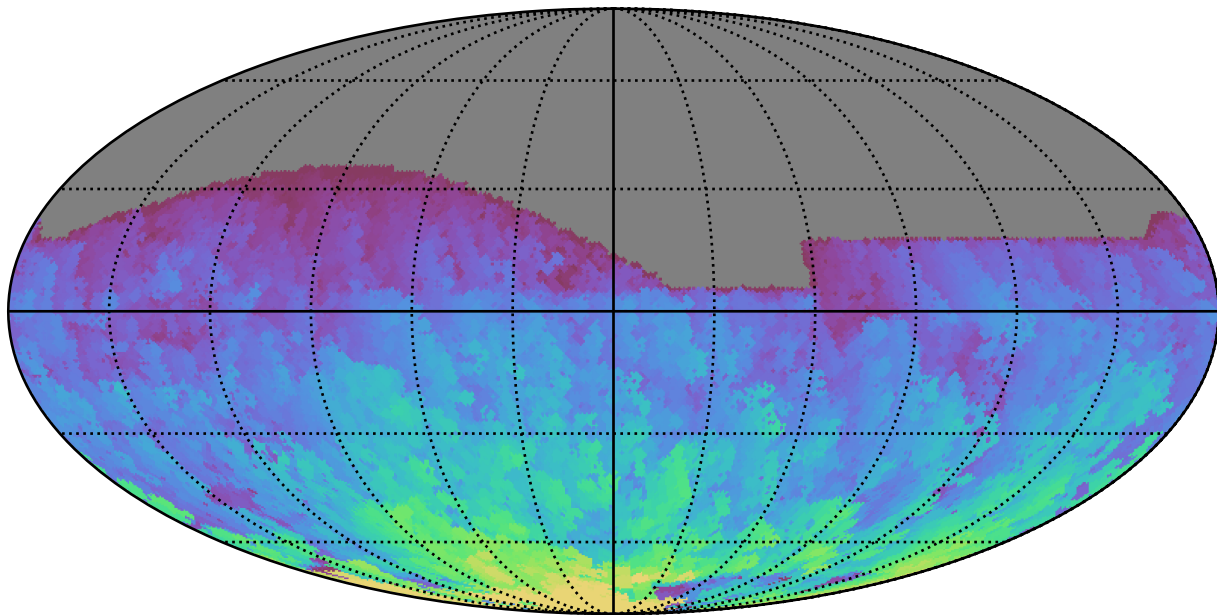
ddf_loaded_half_fl1_v3.4_10yrs All sky r band: Max HA
