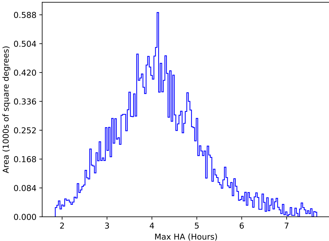
ddf_loaded_half_fl1_v3.4_10yrs All sky r band: Max HA
