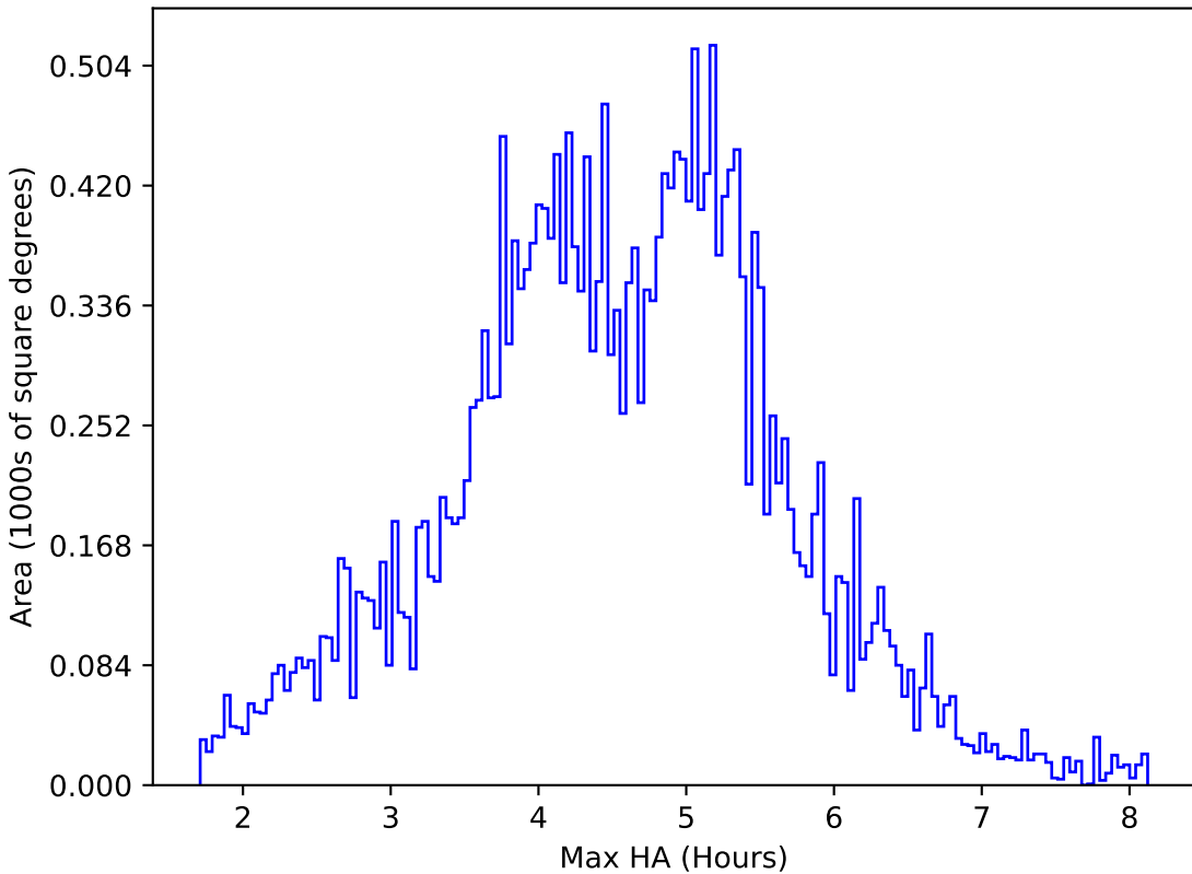
ddf_loaded_half_fl1_v3.4_10yrs All sky i band: Max HA
