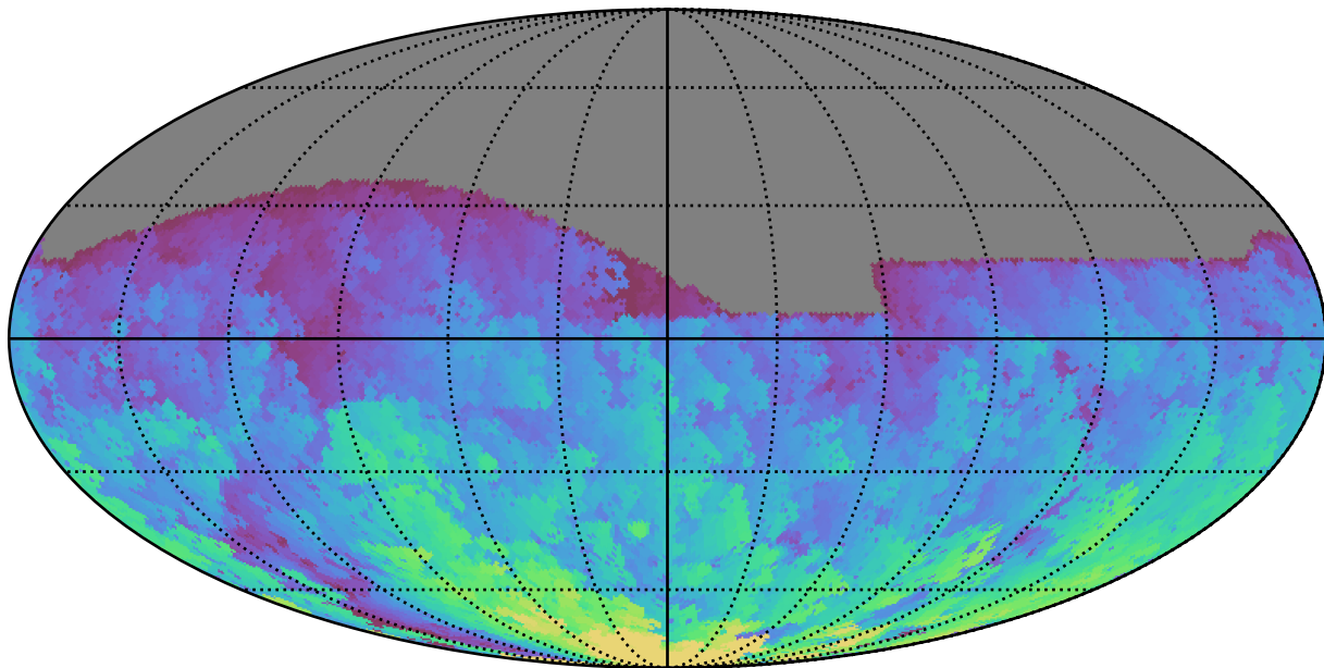
ddf_loaded_half_fl1_v3.4_10yrs All sky g band: Max HA
