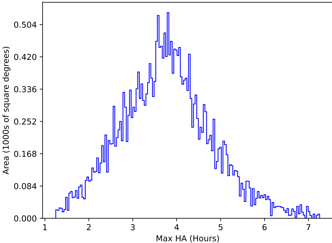
ddf_loaded_half_fl1_v3.4_10yrs All sky g band: Max HA
