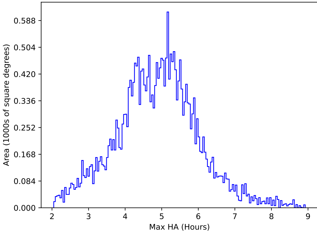
ddf_loaded_half_fl1_v3.4_10yrs All sky all bands: Max HA
