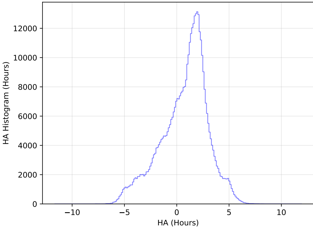
ddf_loaded_half_fl1_v3.4_10yrs WFD z band: HA Histogram
