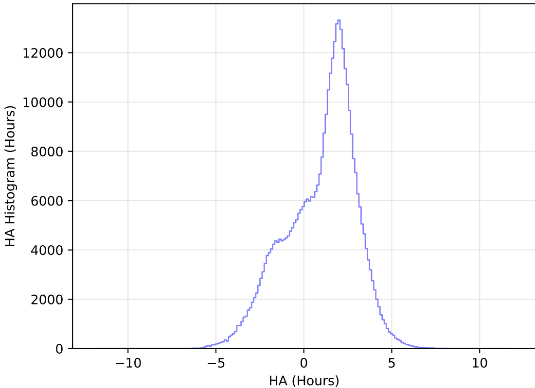
ddf_loaded_half_fl1_v3.4_10yrs WFD y band: HA Histogram
