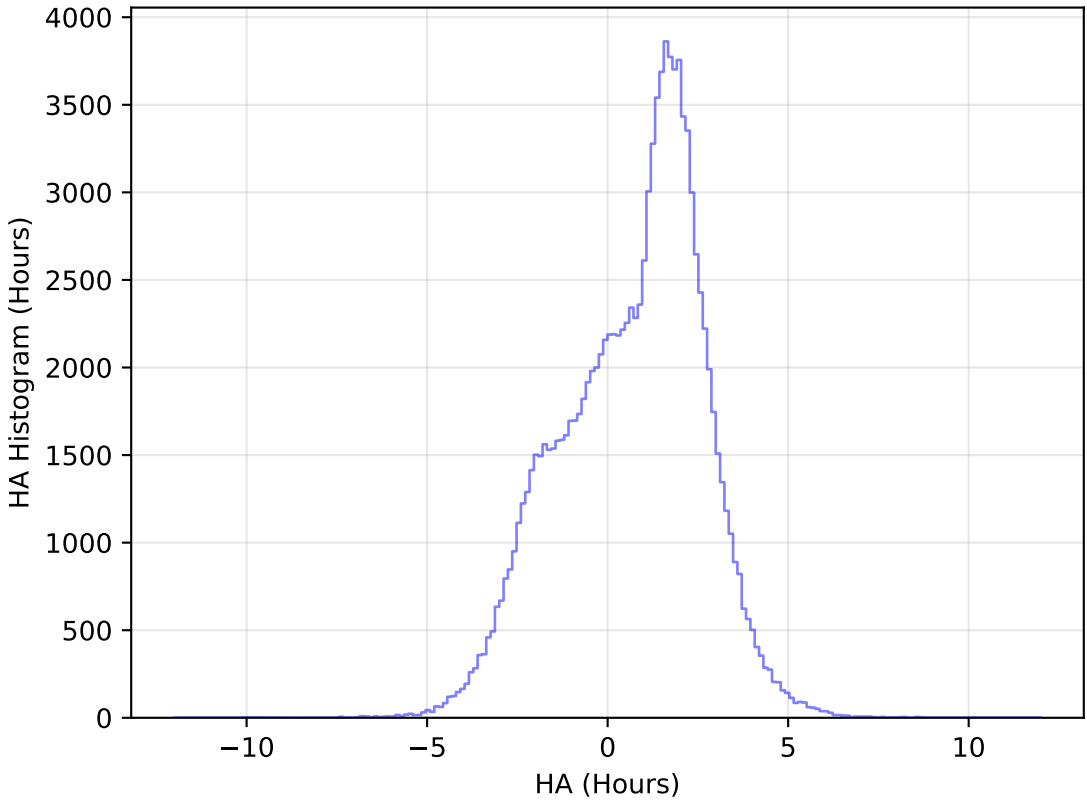
ddf_loaded_half_fl1_v3.4_10yrs WFD u band: HA Histogram
