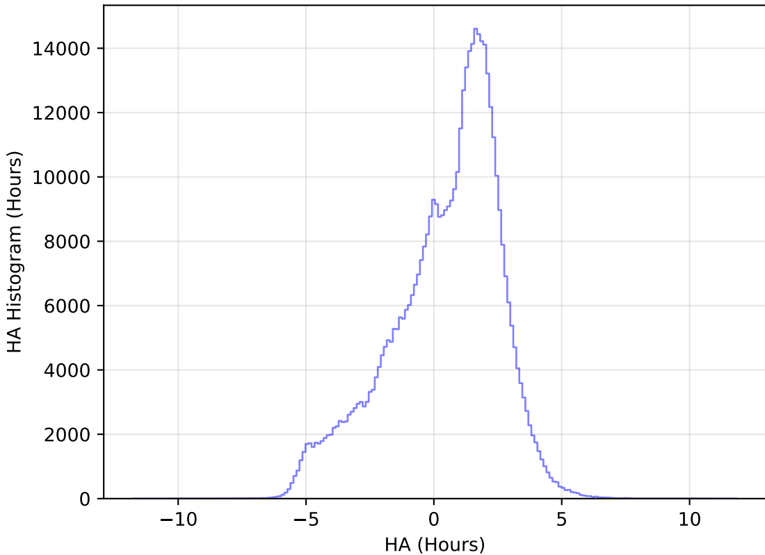
ddf_loaded_half_fl1_v3.4_10yrs WFD r band: HA Histogram
