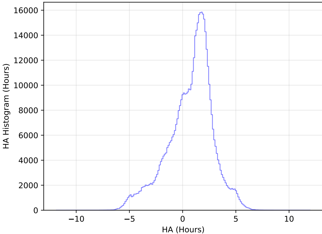
ddf_loaded_half_fl1_v3.4_10yrs WFD i band: HA Histogram
