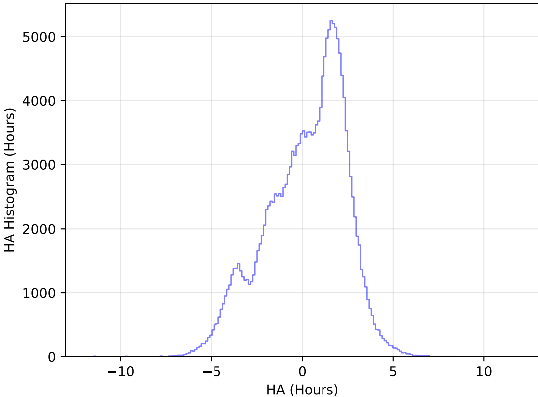
ddf_loaded_half_fl1_v3.4_10yrs WFD g band: HA Histogram
