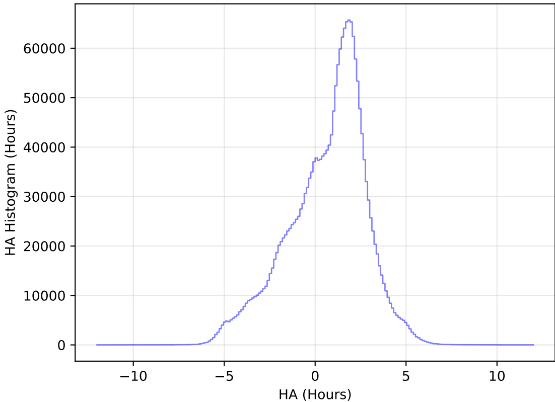
ddf_loaded_half_fl1_v3.4_10yrs WFD all bands: HA Histogram
