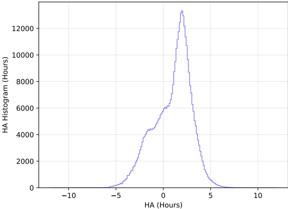
ddf_loaded_half_fl1_v3.4_10yrs All sky y band: HA Histogram
